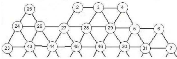
Fig. 5 Reduced graph after visiting start vertex
