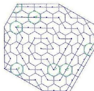
Fig. 8 Cluster Formation
