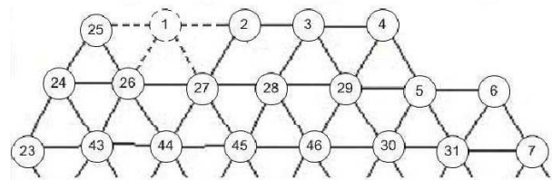
Fig. 4 Start vertex visited
