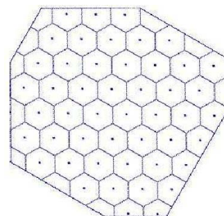
Fig. 7 Hexagonalized area
