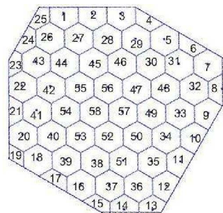
Fig. 2 Hexagonalized region
