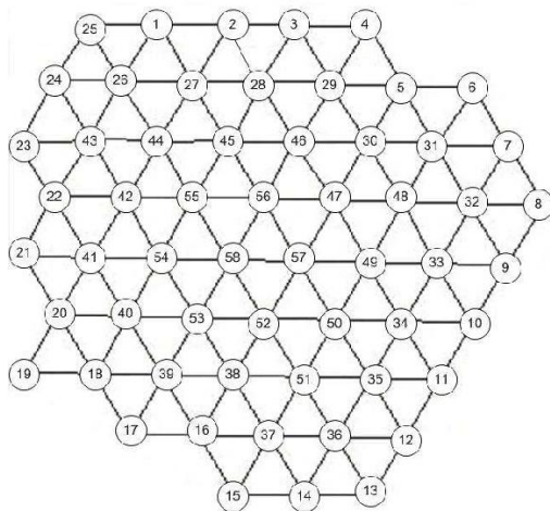
Fig. 3 Underlying graph of hexagonalized region
