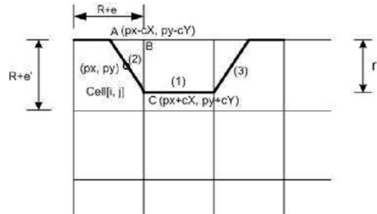
Fig. 1 Hexagon formation
