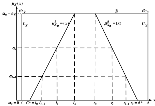
Fig. 3. Trapezoidal fuzzy number
