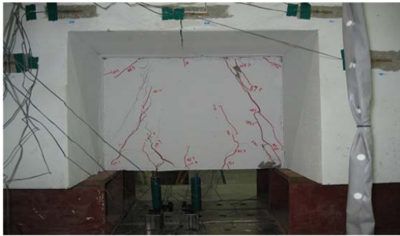
Fig. 12 Crack in SD Type
