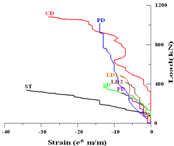
Fig. 13 Strain Curve at C3
