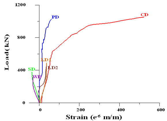
Fig. 15 Strain Curve at S1
