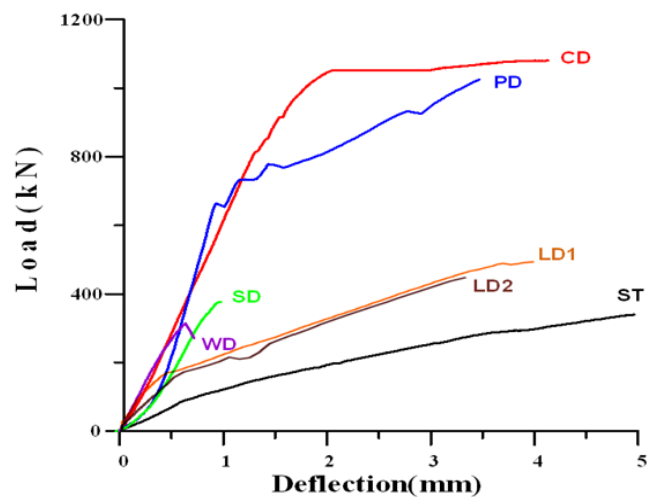
Fig. 7 Load-Deflection Curve at LVDT
