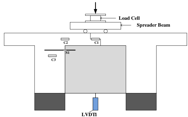
Fig. 6 Location of LVDT and Gauge, Loading
