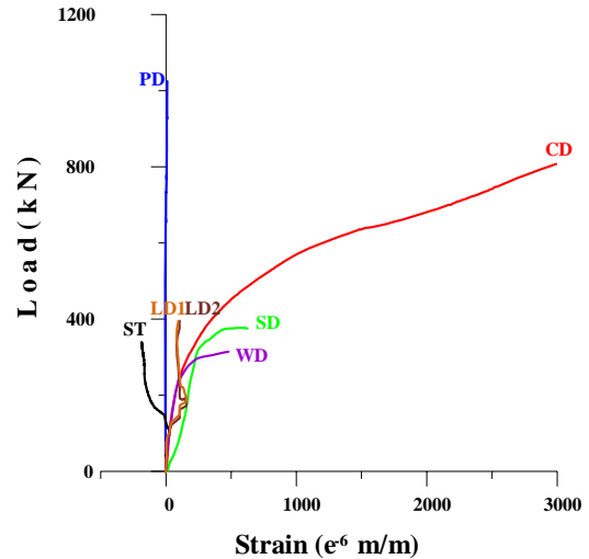
Fig. 9 Strain Curve at C1
