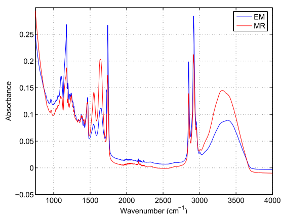
Fig. 1. Average FT-IR spectrum of omental fat samples for Milk Replacer (MR) and Ewe Milk (EM).
