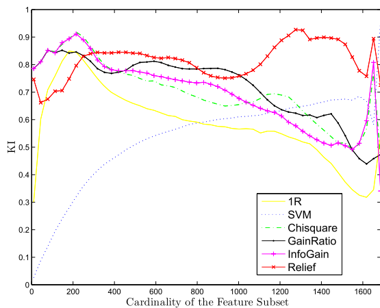
Fig. 2. KI for Feature Subsets with different cardinality
