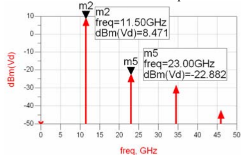
Fig. 6 Harmonics Spectrum
