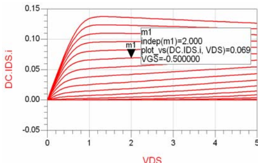
Fig. 4 IV Curve
