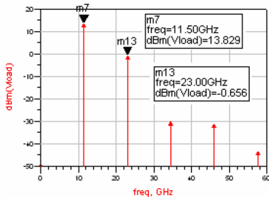
Fig. 17 Harmonics Spectrum
