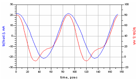
Fig. 12 Output current in time domain before & after filtering
