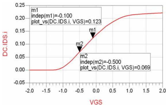
Fig. 3 Transconductance Characteristics
