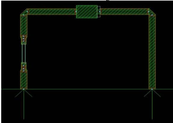
Fig. 21 Layout of Feedback
