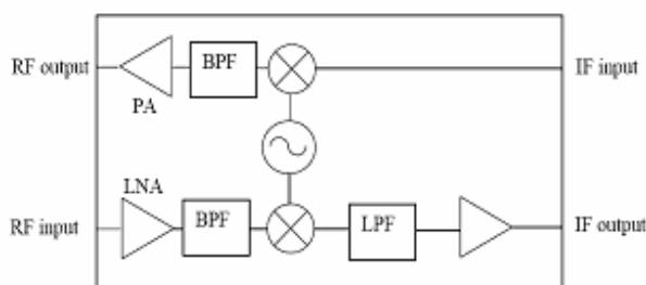
Fig. 1 Transceiver Diagram
