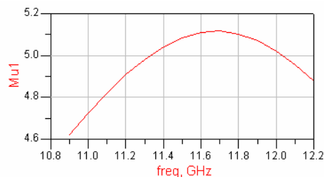
Fig. 14 Stability factor
