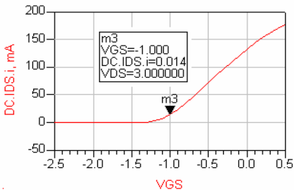
Fig. 9 Transconductance Characteristics
