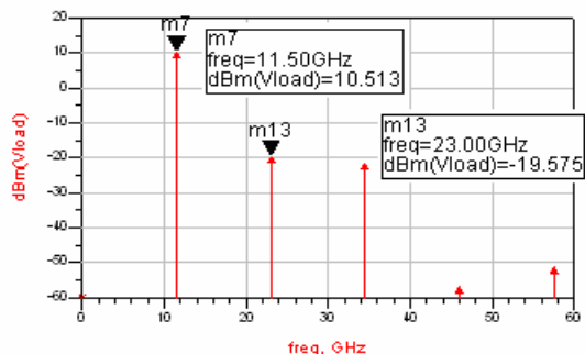
Fig. 11 Output Power
