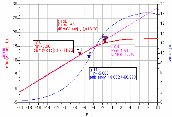
Fig. 15 Large-Signal Nonlinear Performance of PA
