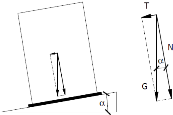
Fig. 2 Slide joint primary testing
