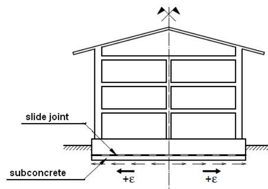
Fig. 1 Schematic drawing of slide joint
