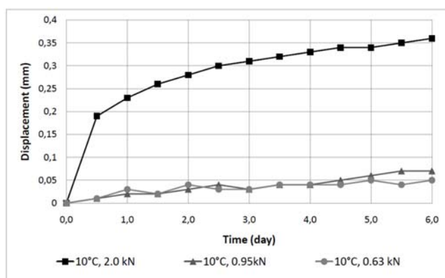
Fig. 6 Measured displacements, 10°C, vertical load 500 kPa
