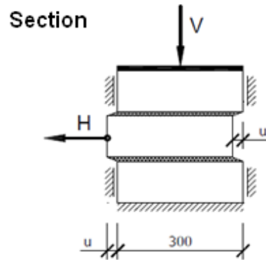
Fig. 4 Schematic drawing of slide joint testing
