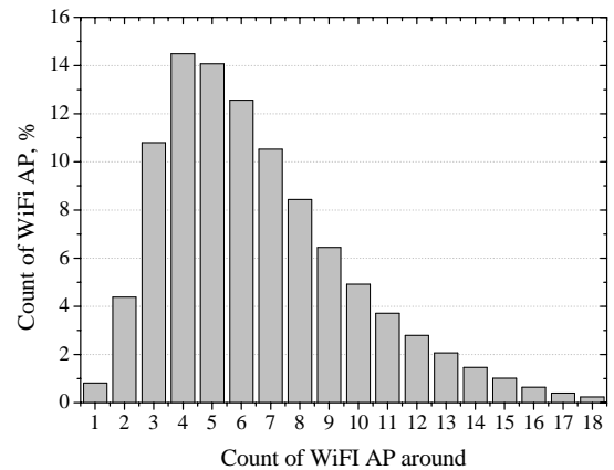
Fig. 5 Histogram of Wi-Fi AP saturation
