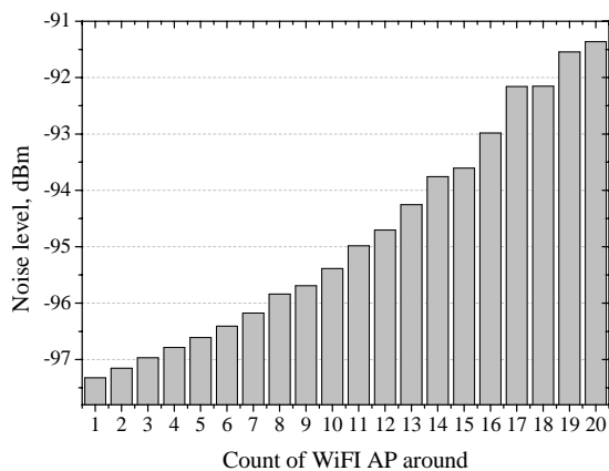
Fig. 7 Wireless noise level histogram
