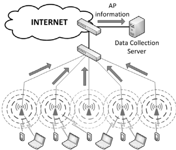
Fig. 1 Structure of wireless monitoring system
