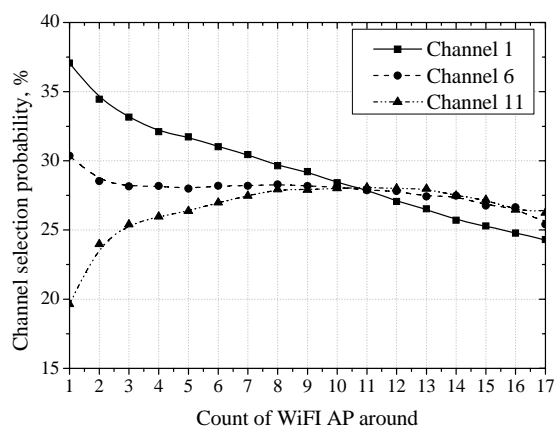
Fig. 6 Channel selection probability based on AP count
