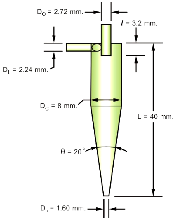
Fig. 1 An 8-mm. diameter Reitema's design hydrocyclone
