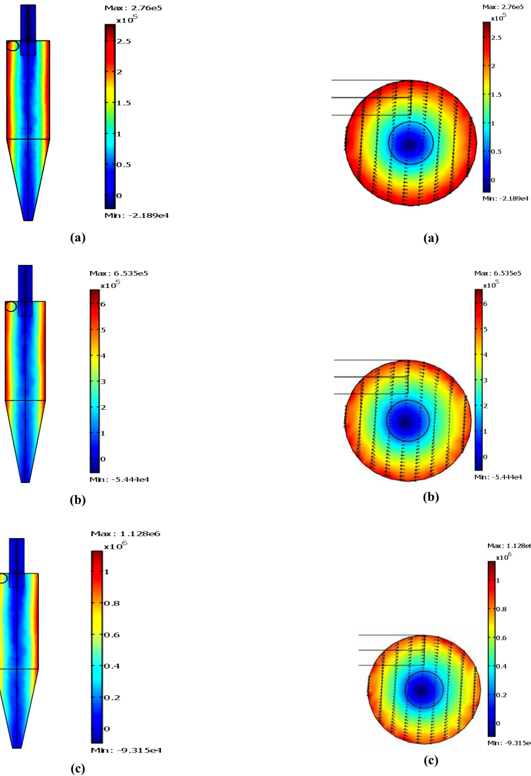
Fig. 7 Pressure distribution on the cross-sectional plane below the opening of vertex finder at different feed pressures: (a) 0.3 MPa, (b) 0.7 MPa, and (c) 1.2 MPa
