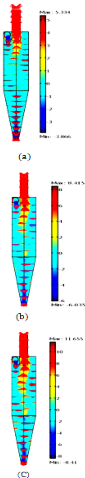
Fig.8 Vertical velocity vector and contour on the axial central plane at different feed pressure: (a) 0.3 MPa, (b) 0.7 MPa, and (c) 1.2 MPa.
