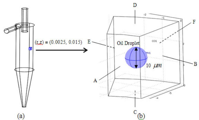
Fig. 2 Computational domains: (a) the entire volume of flow within the hydrocyclone— Domain I , (b) the volume of flow surrounding the 10- \mu\text{m} oil droplet at (r,z) = (0.0025, 0.015) — Domain II .
