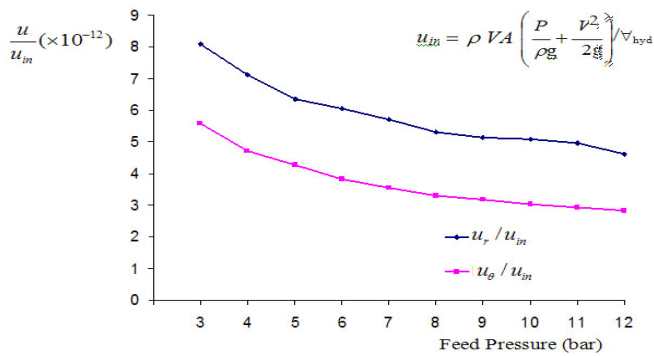
Fig. 17 Energy ratio i.e., strain energy density to feed inlet energy density.
