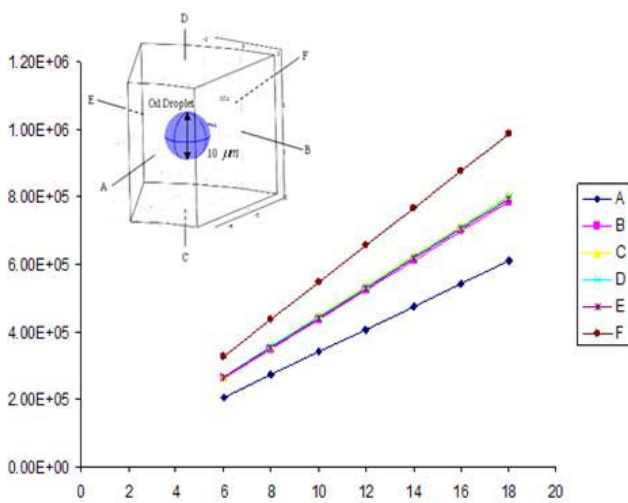
Fig. 4 Local pressure on each boundary of the domain surrounding the 10- \mu m oil droplet
