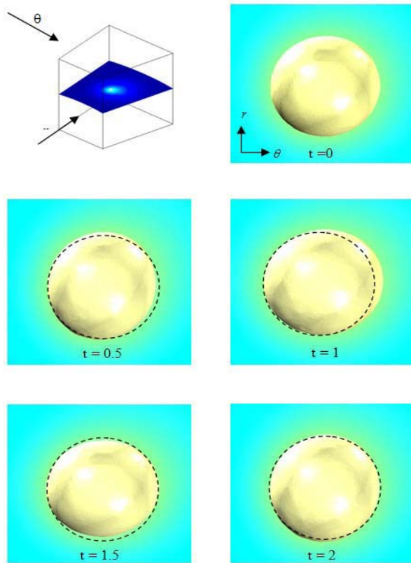
Fig. 10 Time variation of the deformation in the r – and \theta – directions at feed pressure of 0.3 MPa.
