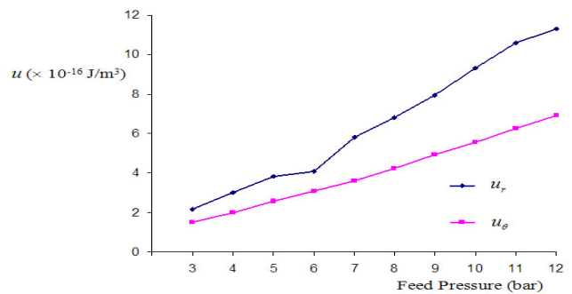
Fig. 16 Strain energy density.
