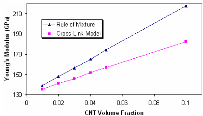
Fig. 3 Young's modulus vs CNT volume fraction
