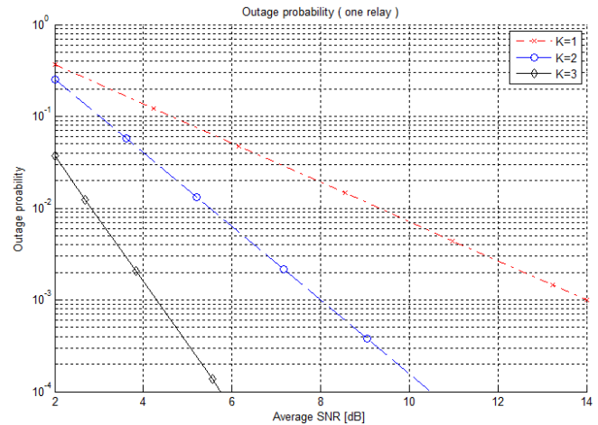
Fig. 2 Outage probability vs. SNR (1 relay)
