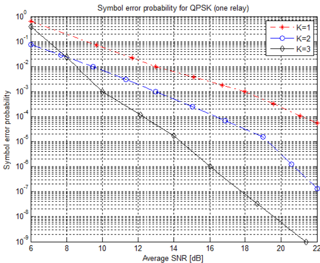
Fig. 4 SEP vs. SNR for one relay
