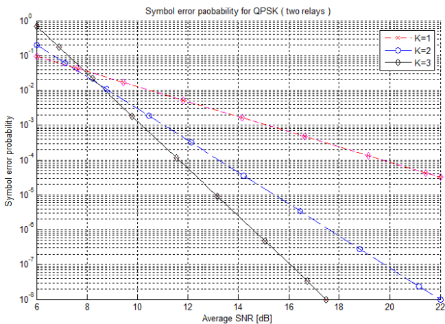
Fig. 5 SEP vs. SNR for two relays
