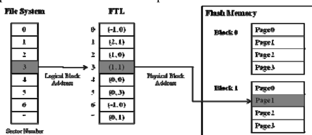
Fig. 1 Page mapping method of FTL
