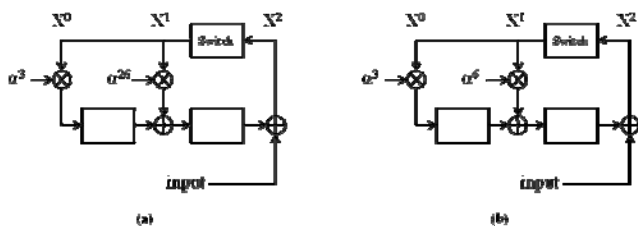
Fig. 5 LFSR encoder for (a) RS(255,253), (b) RS(8,6)
