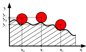
Fig. 2 Point scanning by discontinuous method at CMM [8]
