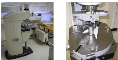
Fig. 7 Measuring device Talyrond 73 and measured part
