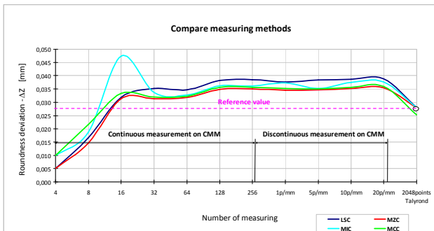
Fig. 8 Graph of the deviations scanned points (for LSC, MZC, MIC, MCC)
