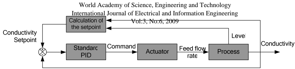
Fig. 1 Bois-Rouge standard control scheme of the C-crystallization process.
