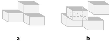
Fig. 1 (a) An OP, (b) An OPP
