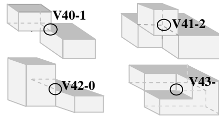
Fig. 4 Four possible vertex configurations for V4
