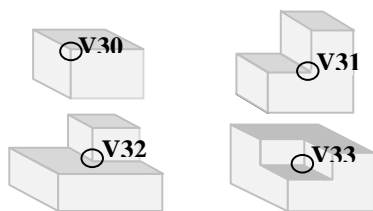
Fig. 3 Four possible vertex configuration for V3
