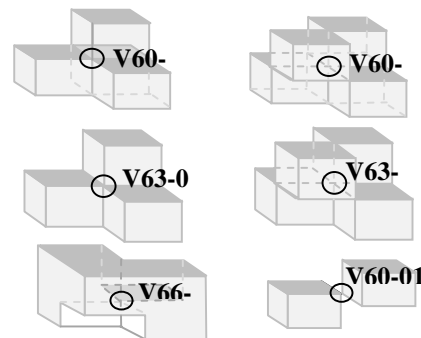
Fig. 6 Configurations a vertex having 6 edges in OPP
