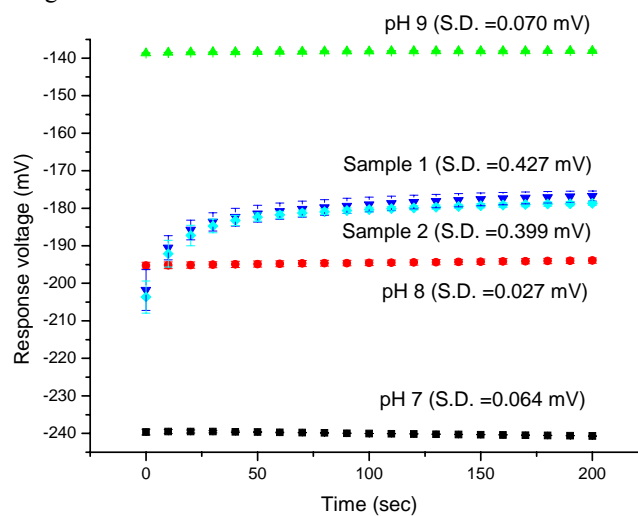
Fig. 4 Short-term responses for pH measurements of sample liquids are between 0 and 200 seconds
