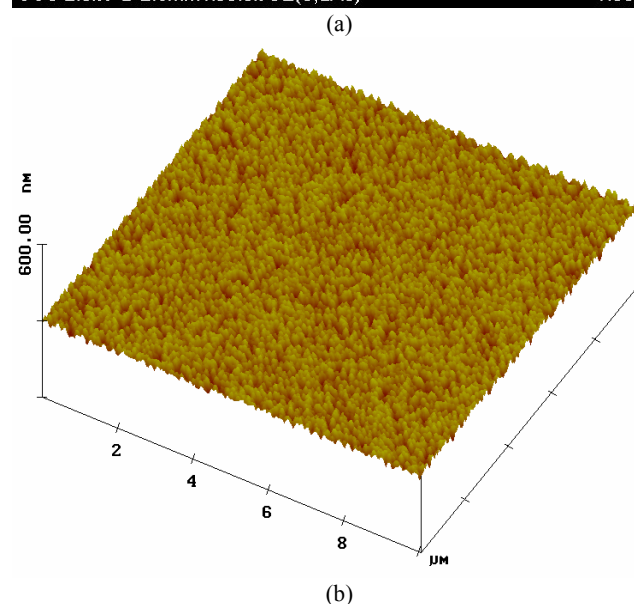
Fig. 2 (a) Surface morphology of TiO 2 :Ru film is measured by FE-SEM; (b) Surface roughness of TiO 2 :Ru film is measured by AFM
