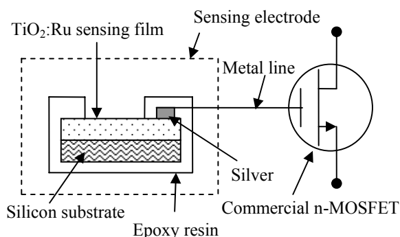
Fig. 1 Structure of TiO 2 :Ru-based separative extended gate field effect transistor (SEGFET) is measured for I-V measurements
