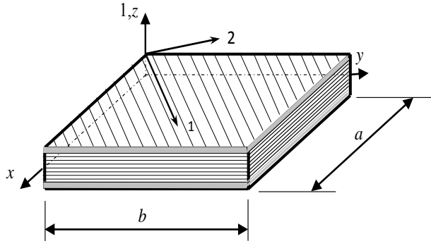
Fig. 2 The shape memory alloy composite plate ( : GE layer, : N-GE)
