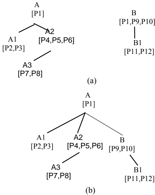
Fig. 2 (a) HPCR trees before fusion (b) Final tree after fusion
