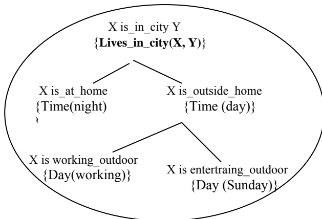
Fig. 1 HPR-tree- Cluster of related HPRs
