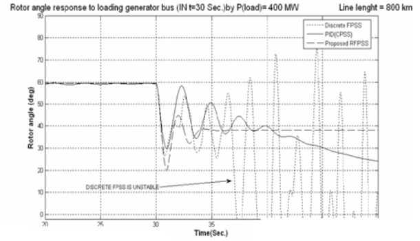
Fig. 11-d P(Load) = 400 MW
