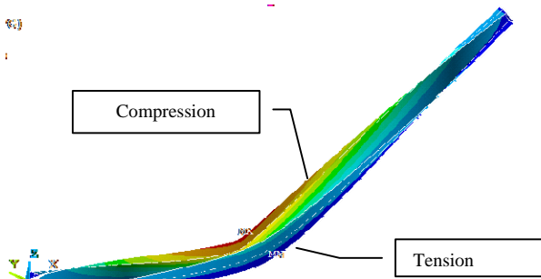
Fig. 5 Excessive Deformations (Post Buckling)
