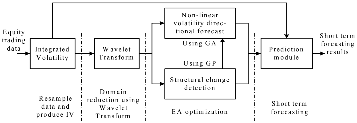
Fig. 1 Proposed volatility directional forecasting system architecture
