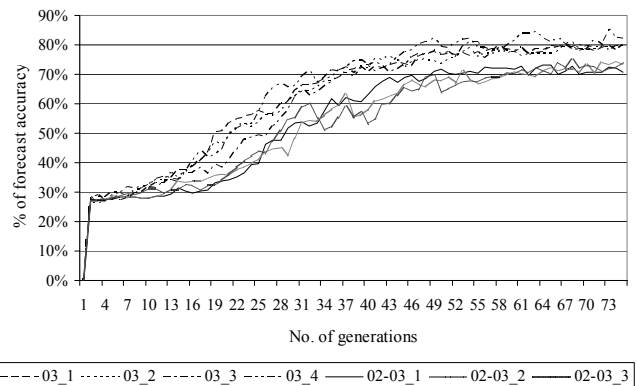
Fig. 5 Daily 2004 S&P500 forecasting accuracy with both 2002/2003 and 2002 data as training data sets
