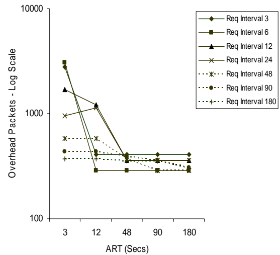
Fig 6a Overhead traffic in 3 minutes by increasing ART for different Request Intervals (5 nodes intercommunicating in 20 node network)
