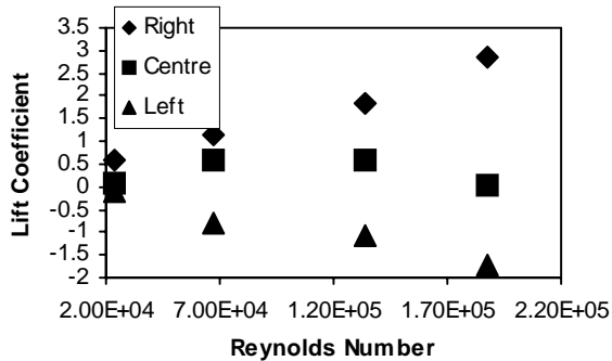
Fig. 9 Variation of Lift Coefficient of Stacks in Side-by-side Configuration
