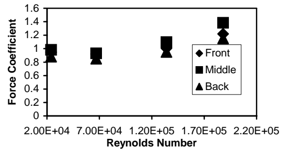
Fig. 6 Variation of Total Force Coefficient of Stacks in Linear Along Wind Configuration
