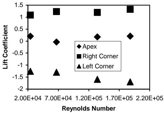
Fig. 13 Variation of Lift Coefficient of Stacks in Triangular Configuration
