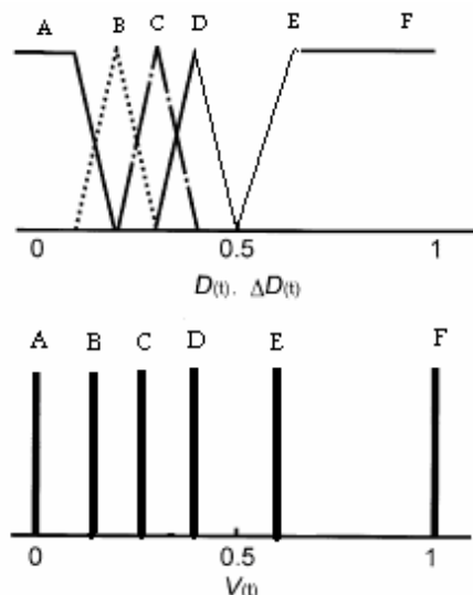
Fig. 3 Membership functions for fuzzy logic
