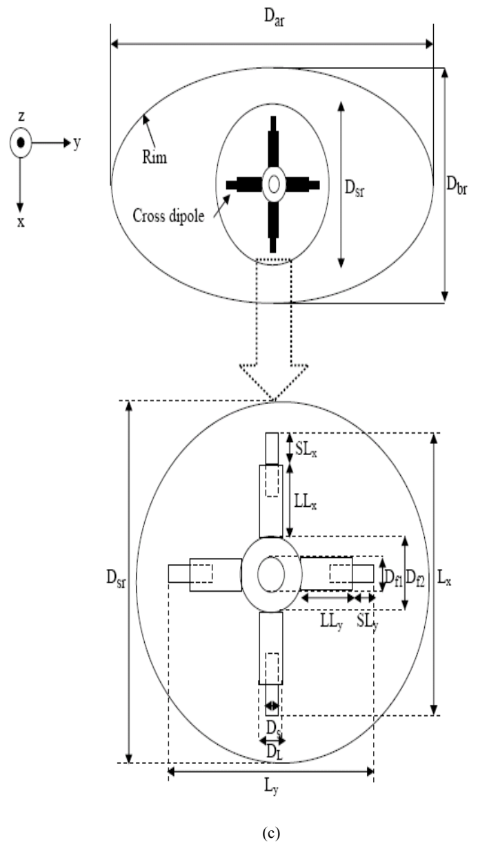
Fig.1 Short backfire antenna excited by cross dipole (a) 3-D view (b) Side view (c) Top view
