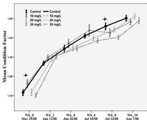
Fig. 5 Mean ( \pm S.E.) condition factor [ 100(\text{weight} \cdot \text{length}^{-3}) ] of rainbow trout fed varying dosages of Fin-Immune TM at week 0 (start) to week 6. At week 7, all fish received the control diet (0 mg Fin-Immune TM ) until week 10. Symbols (+) indicate significant difference from others at that week.
