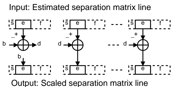
Fig. 7. Floating-point based scaling technique implementation
