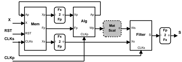
Fig. 1. Block diagram of BSS block processing
