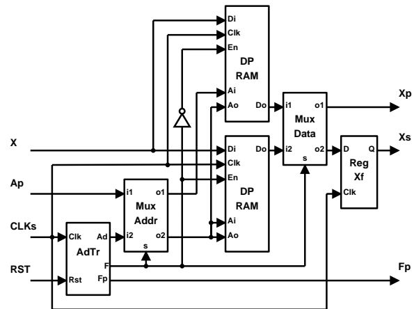
Fig. 3. Memory system block diagram
