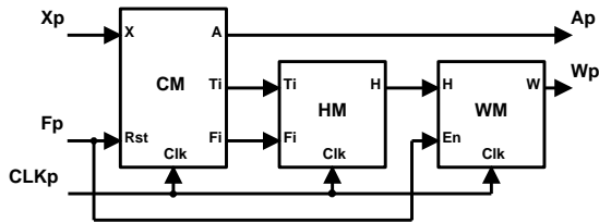
Fig. 4. ASOBI implementation block diagram
