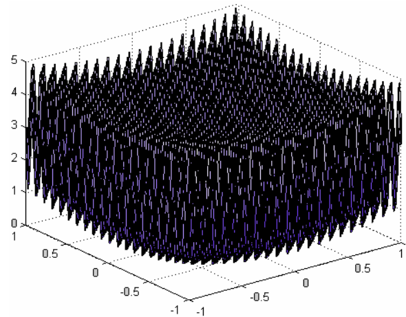
Fig. 2 The Bohachevski function in [-1,1]
