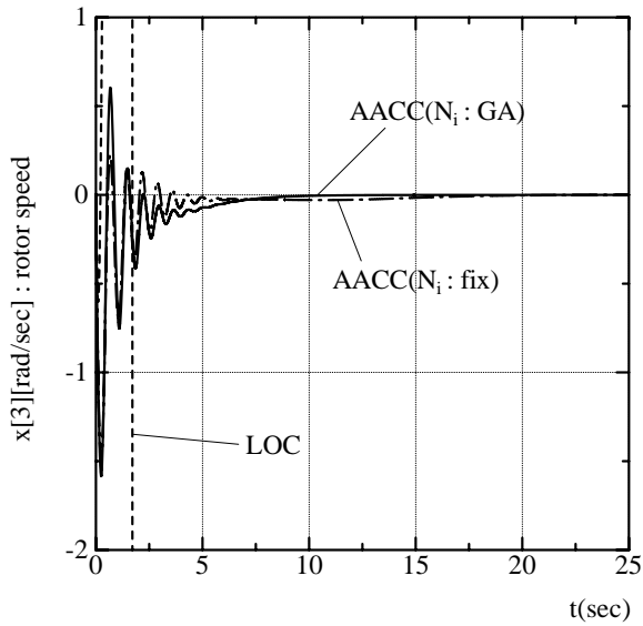
Fig. 6 Responses of LOC, AACC( N_i : fix), AACC( N_i : GA) ( x^T(0) = [0, 1.2, 0] )
