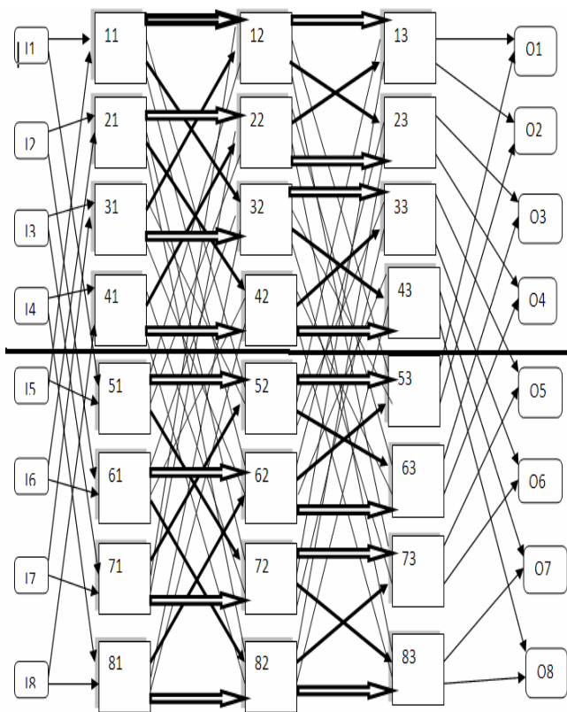
Fig. 7 Structure of two layer 8X8 IBSF
