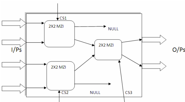
Fig. 10 Microstructure of Output Stage Switching Block
