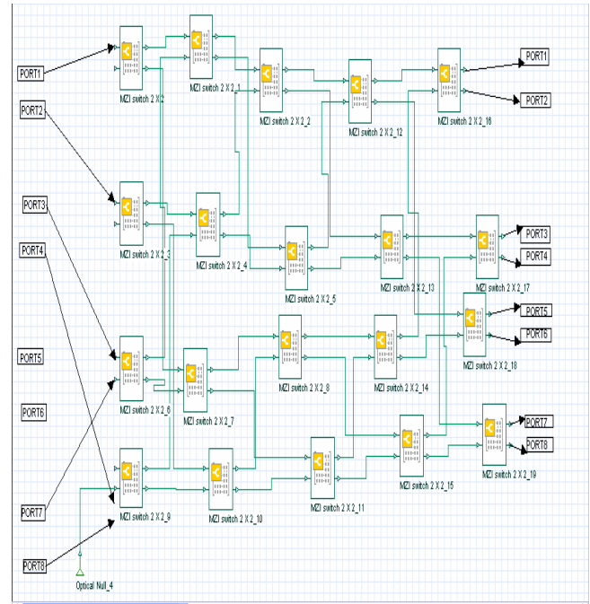
Fig. 6 The modified Banyan Network (8 X 8) of MZI switches clearly showing the input ports {left set} and output ports {right set} of the network with horizontal expansion of 2 extra stages (courtesy OptiSystem module of optiwave software)
