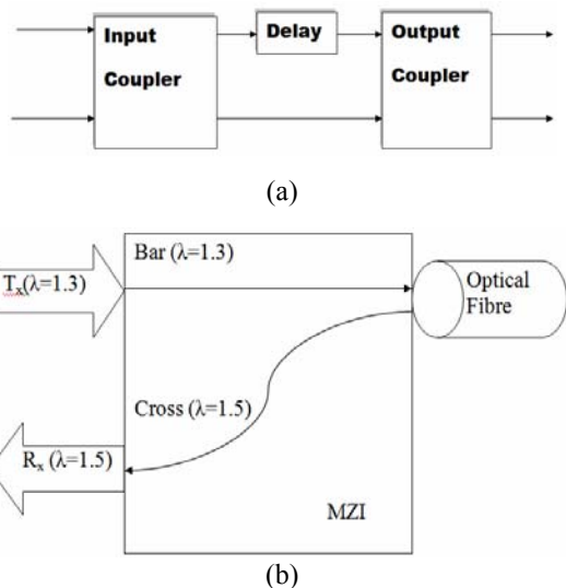
Fig. 1 Layout of (a) structure and (b) functioning of MZI with unequal interferometric arms
