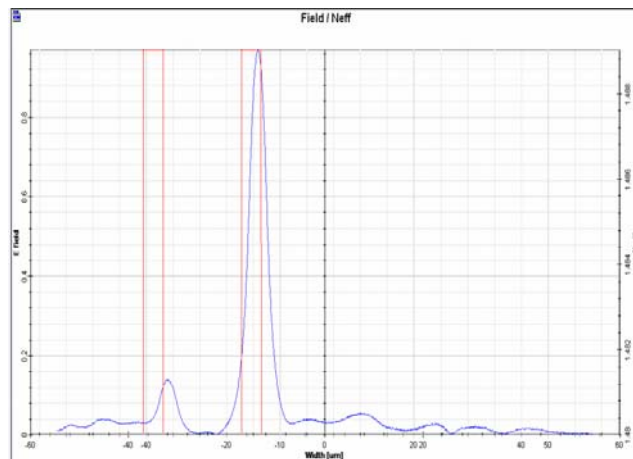
Fig. 3 The graph plotted with variations in relative field strength and the effective refractive index of the waveguide with the width of the wafer used in the switch architecture (courtesy optiBPM module of Optiwave software)
