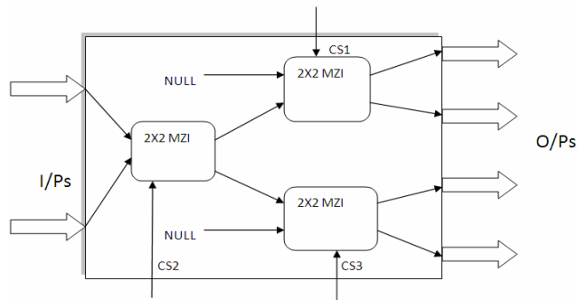
Fig. 8 Microstructure of Input Stage Switching Block
