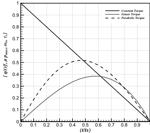
Fig. 4 Variation of [q(t)/f_c \mu p_{\max o} \omega_{ro} r_i] with (t/t_s) for constant, linearly and parabolically increasing torque
