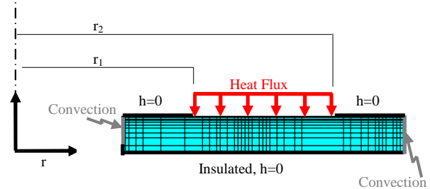
Fig. 5c FE model with boundary conditions for cases (2 & 3)
