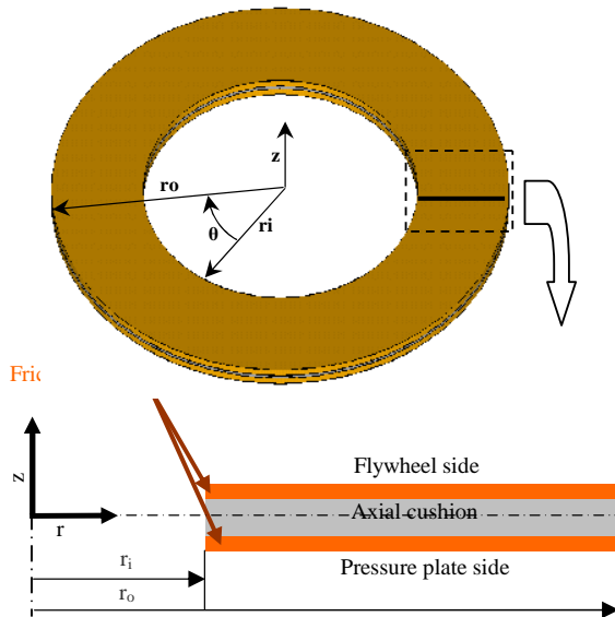
Fig. 5a The friction clutch disc (axisymmetric)
