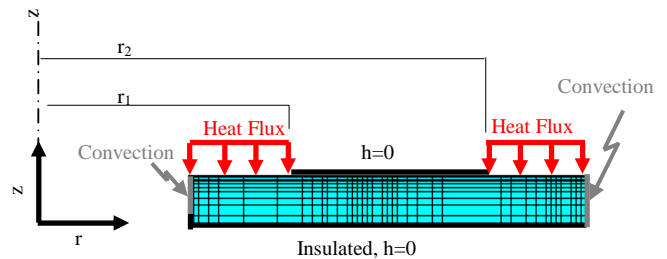
Fig. 5c FE model with boundary conditions for cases (2 & 3)
