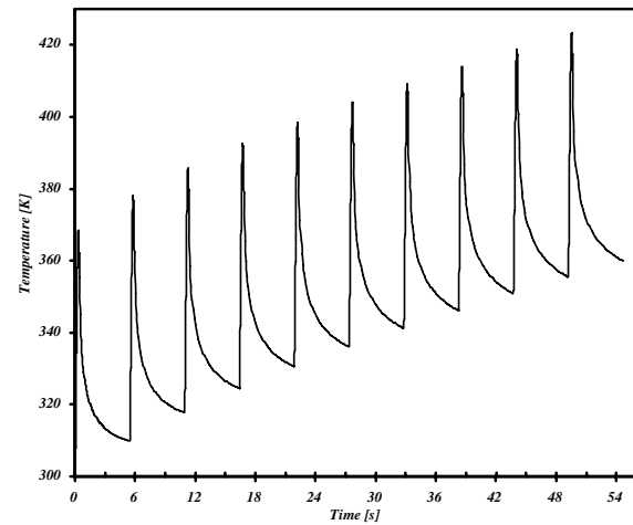
Fig. 15 Variation of temperature with time at r_m (Repeated engagements- parabolic pressure- case 2)
