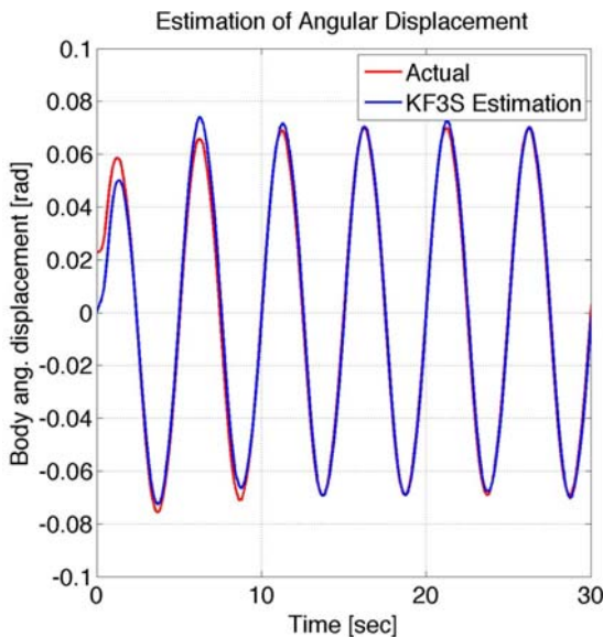
Fig. 6 Measured and estimated body angular displacement.
