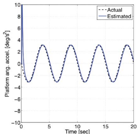
Fig. 13 Estimated and actual ground angular acceleration as obtained by the extended disturbance observer
