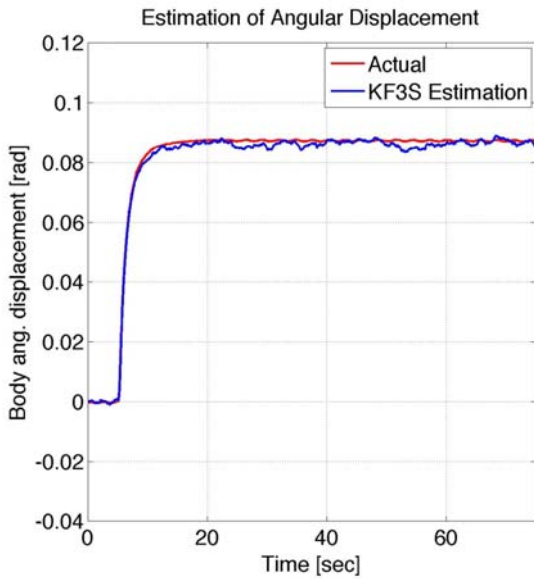
Fig. 5 Measured and estimated body angular displacement.
