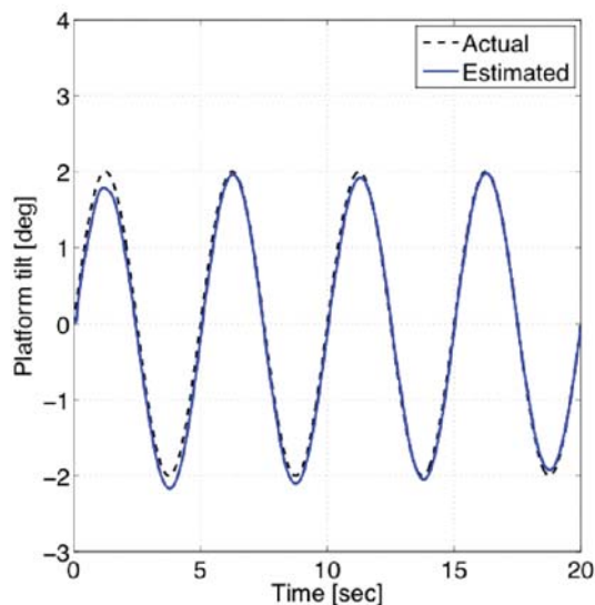
Fig. 9 Estimated and actual platform inclination as obtained by the stand-alone Kalman filter
