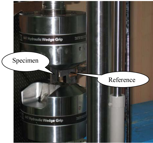
Fig. 3 Specimen mounting details for IRT test
