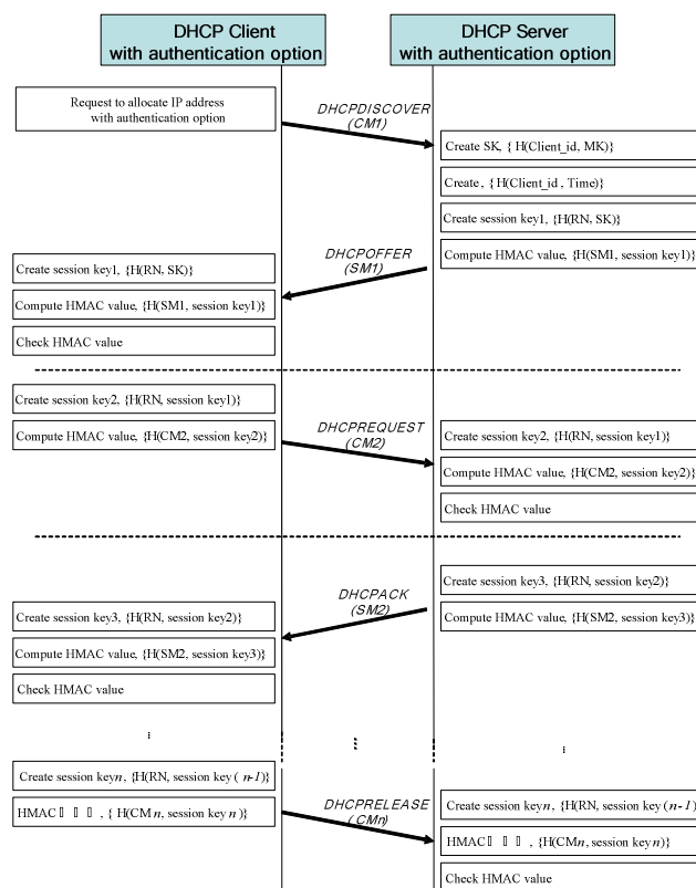
Fig. 4 Processing of message interaction with authentication option
