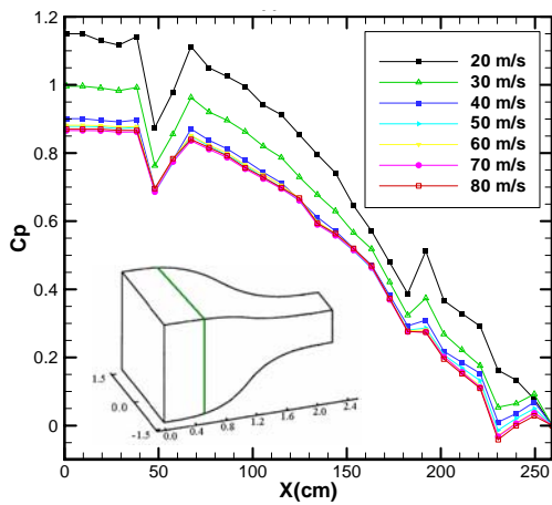
Fig. 9 Cp distribution along the contraction for case 3
