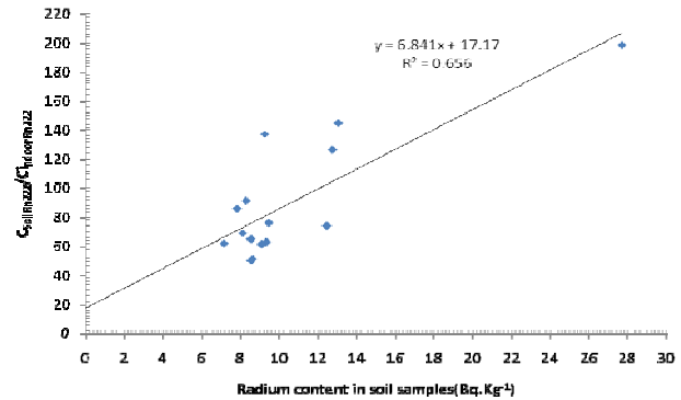
Fig. 3 Variation ratio of soil to indoor radon concentration with the radium content in soil samples.
