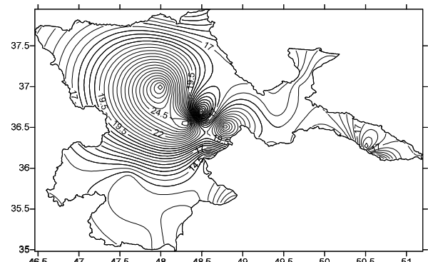
Fig. 6 Maximum means temperature in Sefid-rud basin in 1999
