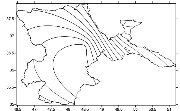
Fig. 7 Minimum means temperature in Sefid-rud basin in 1957
