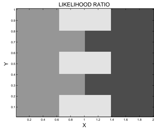
Fig. 9. Optimal decision areas corresponding to ER = 9.4% obtained with true likelihood ratio.
