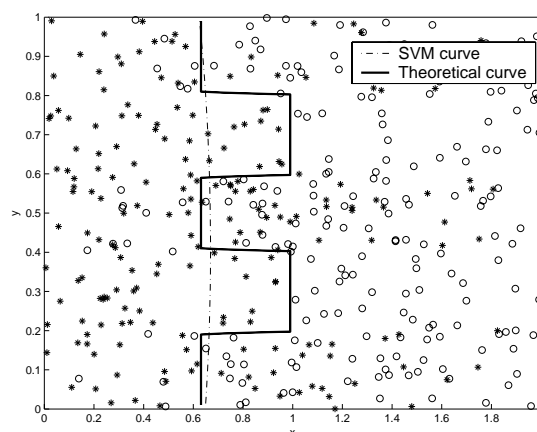
Fig. 6. Partitions corresponding to FPR= 0.1.
