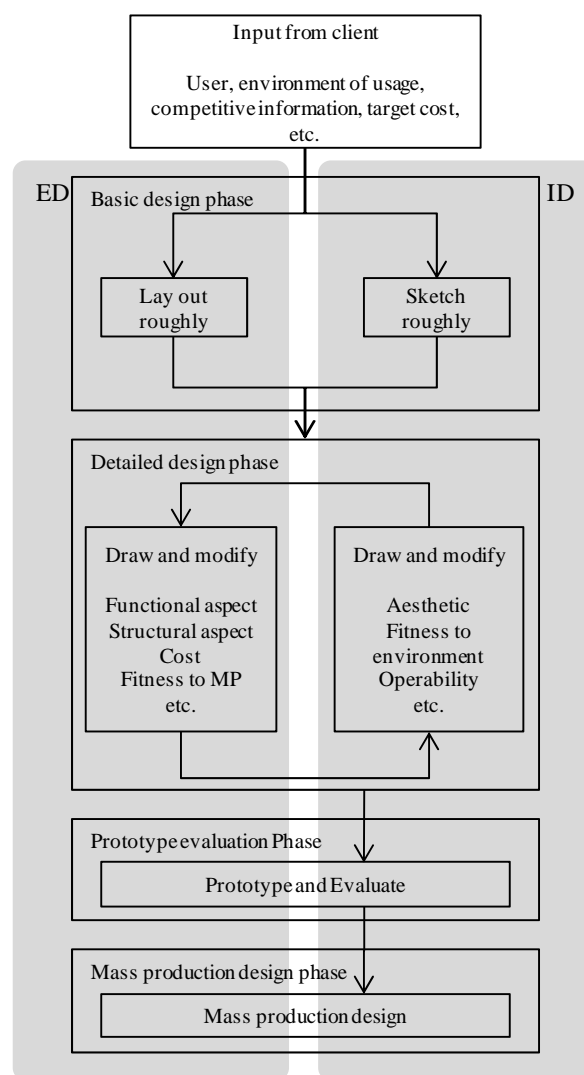
Fig. 1 Integration process
