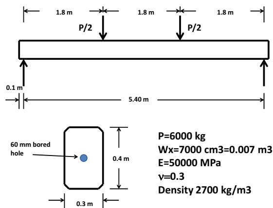
Fig. 8 Test arrangement
