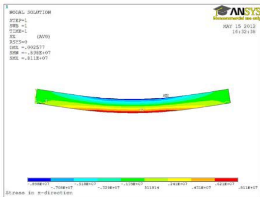
Fig. 9 Stress distribution in the beam according to the FEM analysis
