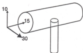
Fig. 2 bSchematic picture of a bored repository tunnel with 5 m diameter and about 8 m deep canister deposition hole with 1.7 m diameter extending from it. The highest primary rock stress 30 MPa is horizontal and oriented perpendicularly to the tunnel axis
