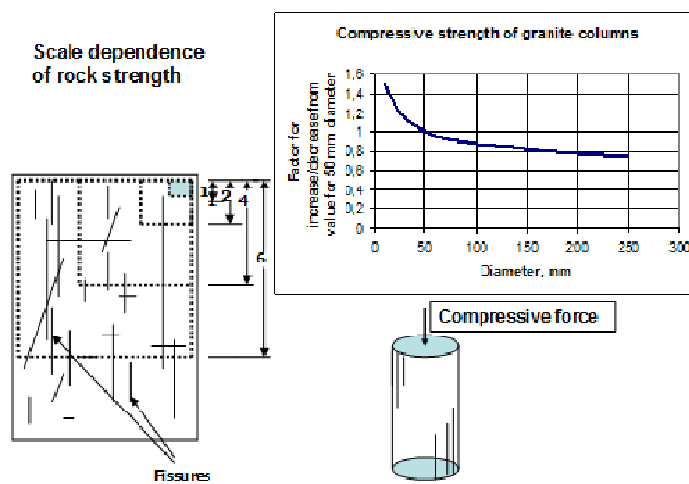
Fig. 7 Influence of size of sample with one type of defects on the compressive strength. The drop in strength at increased volume is explained by the increasing number of defects and the greater possibility of critical orientation and interaction of the defects [1].
