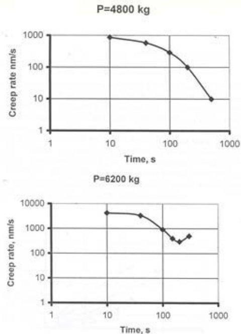
Fig. 11 Creep rates for P=48 kN (4800 kg) in the upper diagram and 62 kN (6200 kg) in the lower. For the first mentioned load the creep rate was still obvious after 10 minutes and for the last mentioned load “tertiary” creep started soon after load application and led to failure after a couple of minutes.
