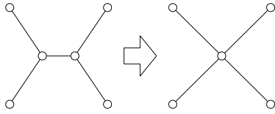
Fig. 1. An example of edge contraction operations.
