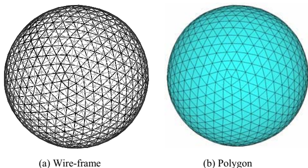
Figure 10. The result of pressing “dttdttdt” for an icosahedron
