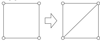
Fig. 3. An example of diagonal addition operations.
