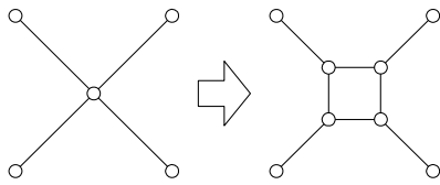
Fig. 2. An example of vertex splitting operations by the present definition in this paper.
