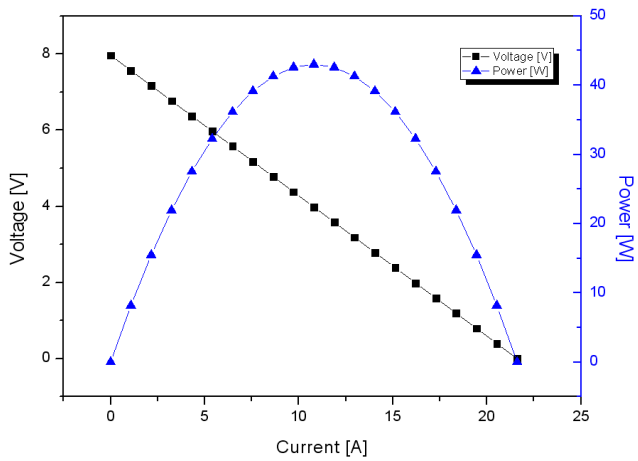
(e) Engine speed: 3000 rpm
