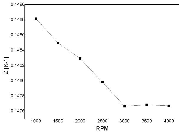
Fig. 5 Figure of merit
