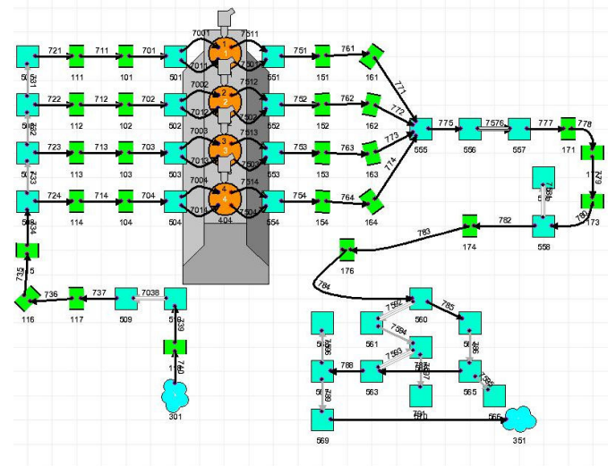
Fig. 1 Diagram of simulation modeling
