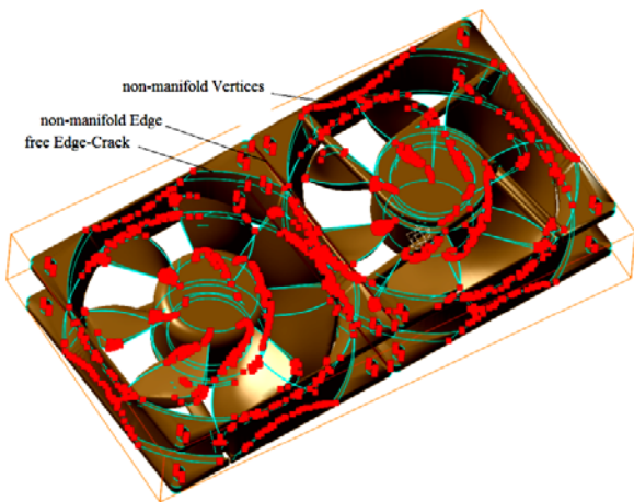
Fig. 8 Bad STL model
