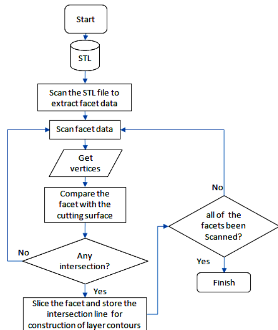
Fig. 3 Slicing Algorithm
