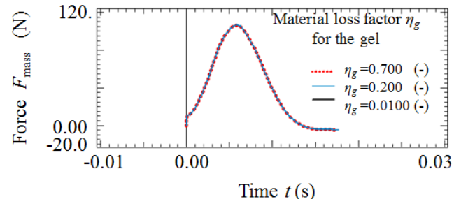
Fig. 15 Effects of material loss factor \eta_g of the gel on the reference force F_{mass}
