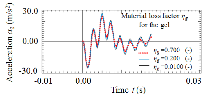
Fig. 16 Effects of material loss factor \eta_g of the gel on dynamic errors of the force transducer
