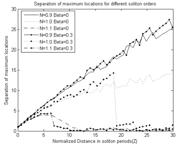
Fig. 8 Separation between the maximum locations of the two polarizing components \Delta T_{peak}(Z) for different soliton orders N and \beta with \delta=0.5
