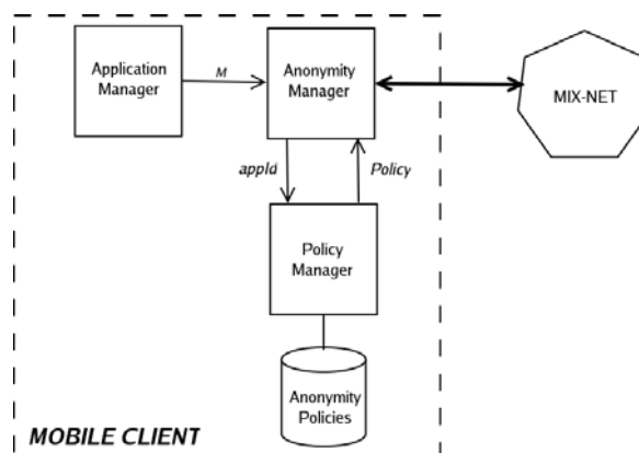
Fig. 4 Architecture of Dynamic Anonymity Framework
