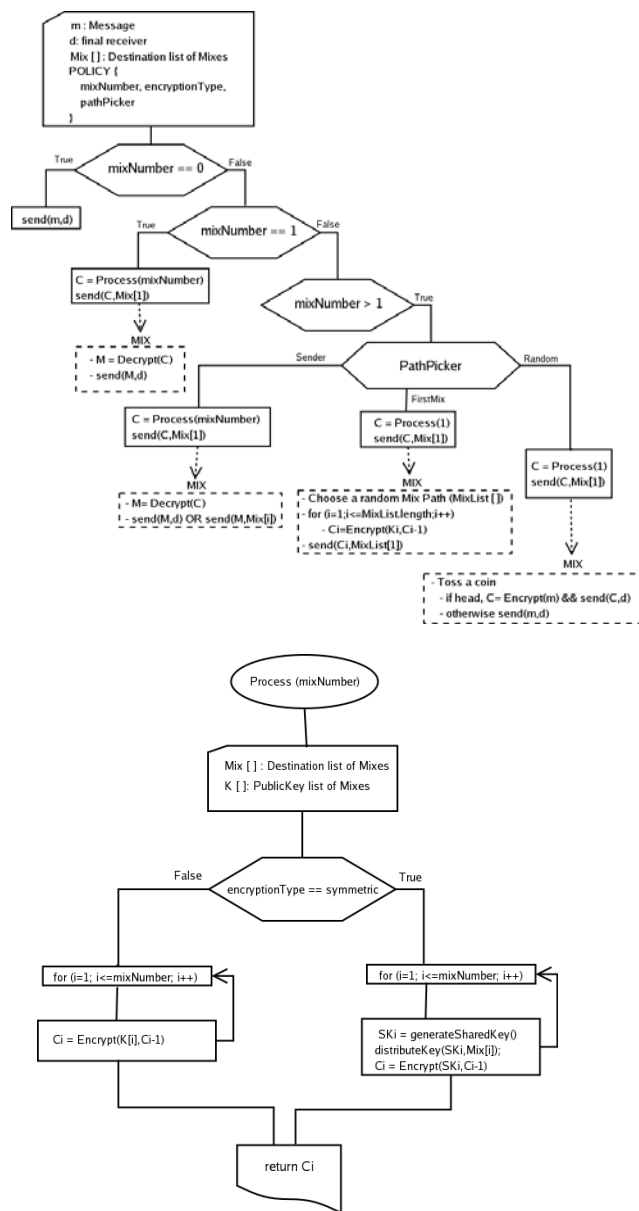
Fig. 5 The Algorithm over Policy
