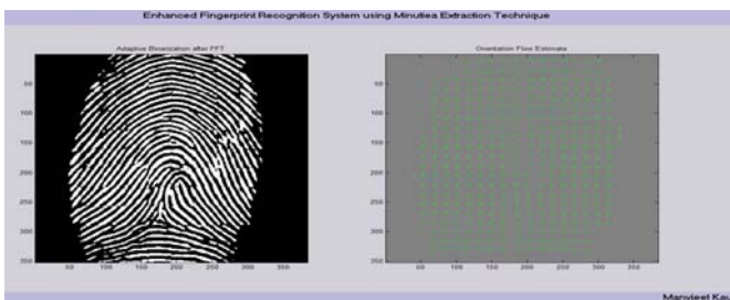
Fig. 9 Direction map. Binarized fingerprint (left), Direction map (right)
