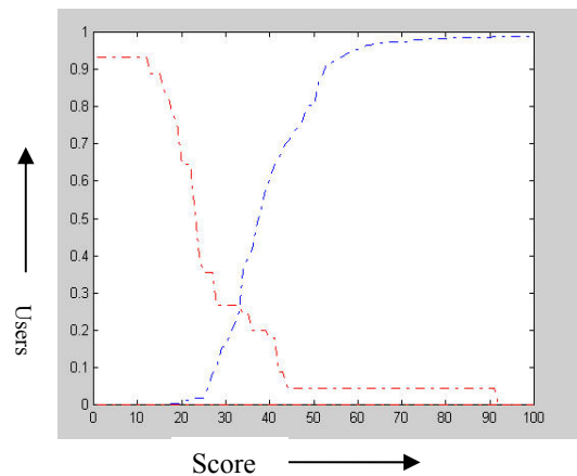
Fig. 13 FAR and FRR curve Blue dot line: FRR curve Red dot line: FAR curve
