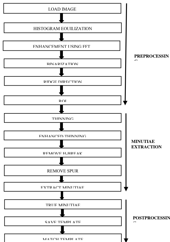
Fig. 3 Algorithm level Design
