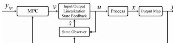
Fig.4: The GLC-output feedback structure
