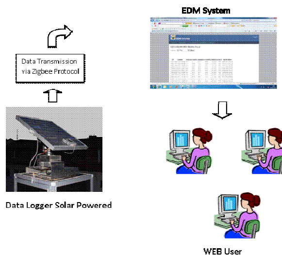
Fig. 3 System Configuration
