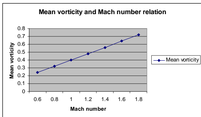
Fig. 4 Mach number and mean vorticity relation
