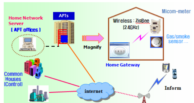
Fig. 4. Network Configuration of a Gas Safety Management System
